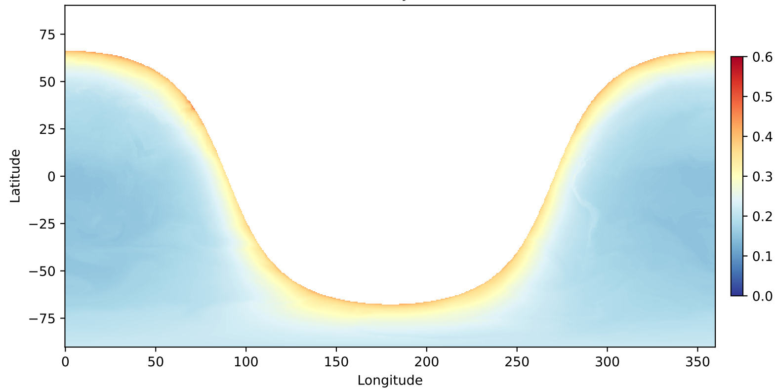
(c) Planetary Albedo
