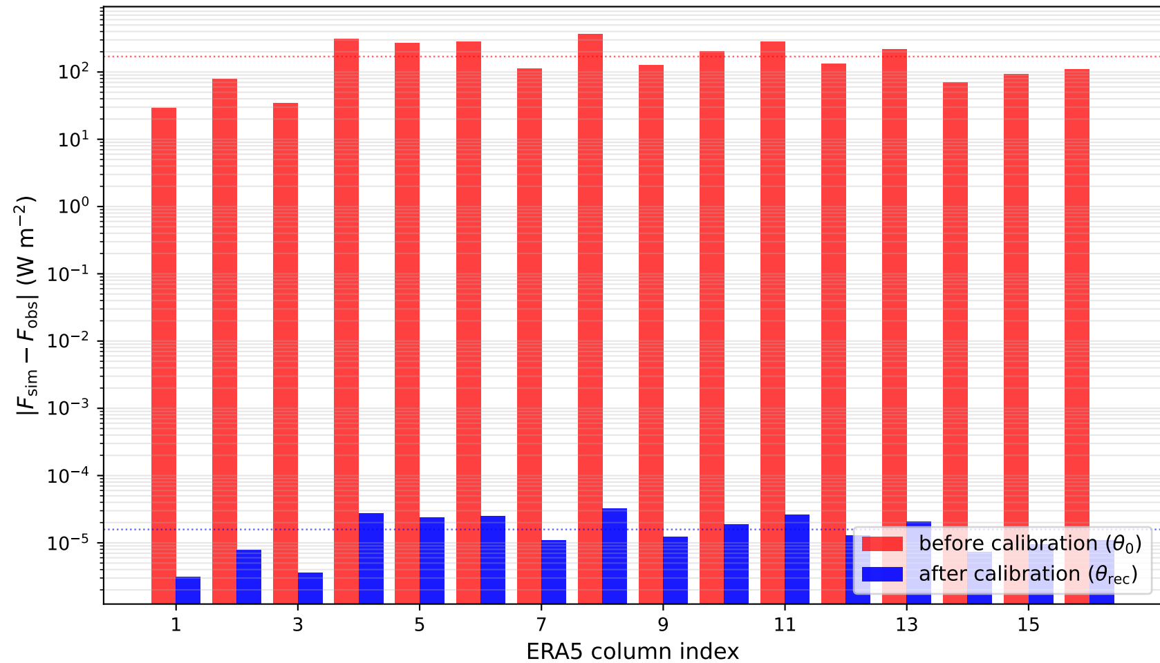
Per-column surface SW flux residual: before vs after 2-D calibration
