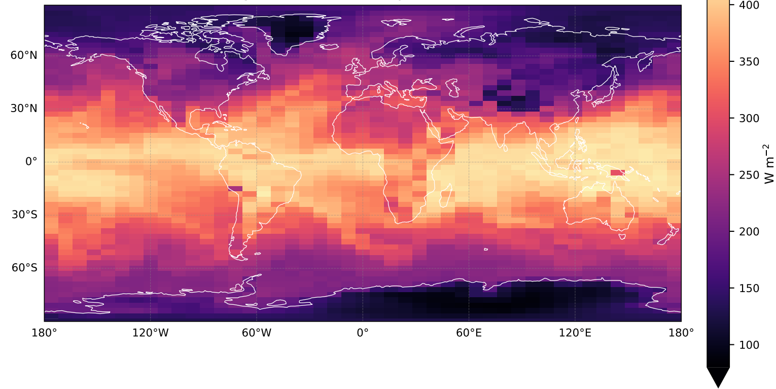
(b) Surface Downward Longwave Flux (Clear Sky)
