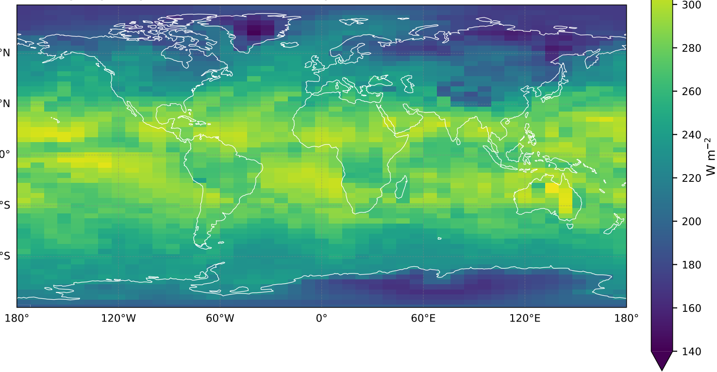
(a) Outgoing Longwave Radiation (Clear Sky)
