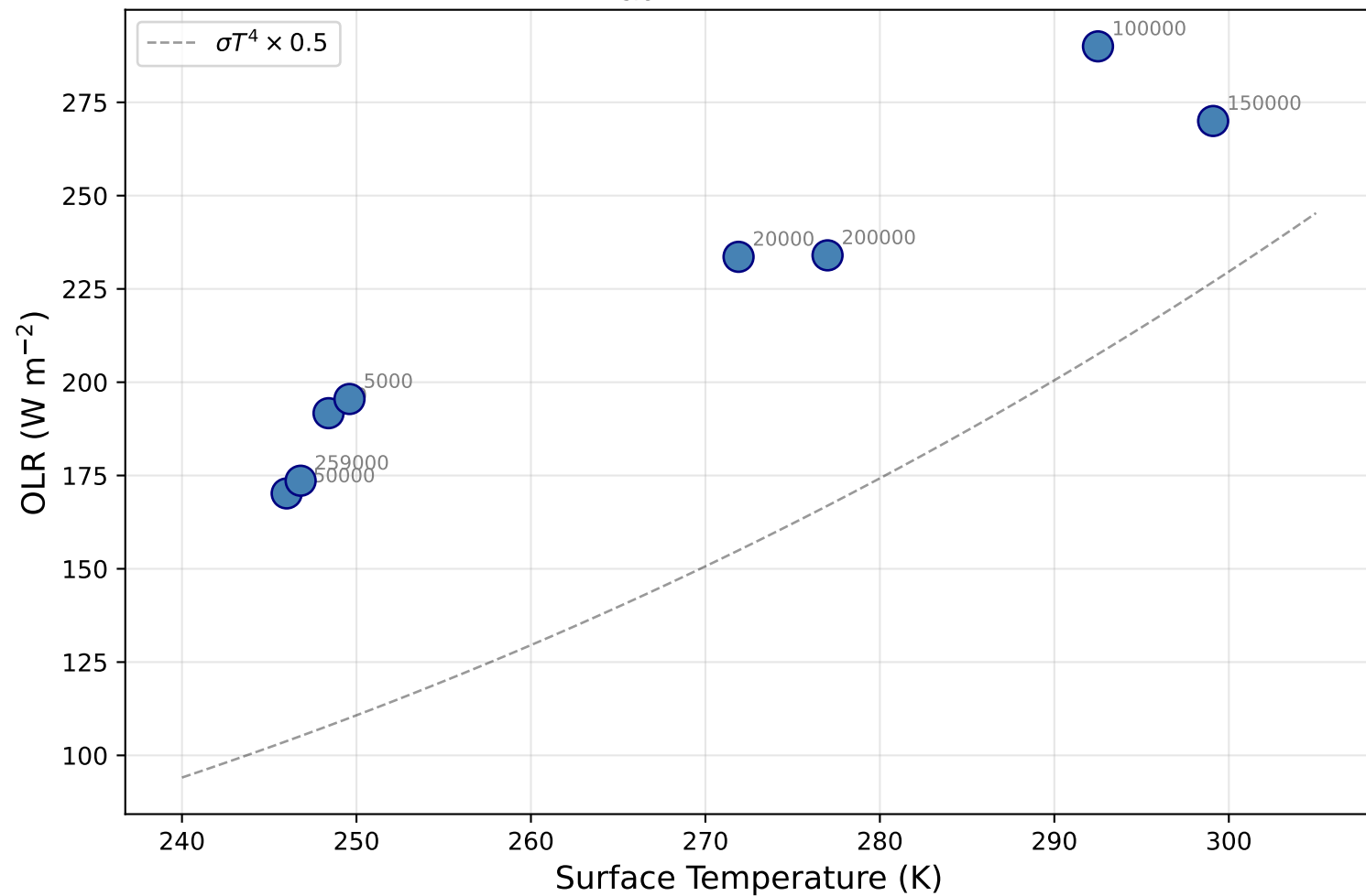
(a) LW OLR vs T_{\text{sfc}} (8 ERA5 columns, 137 levels)
