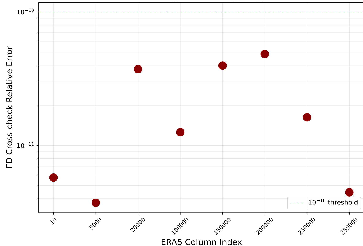
(b) Autograd vs FD: \partial F_{\text{OLR}} / \partial T_{\text{sfc}}
