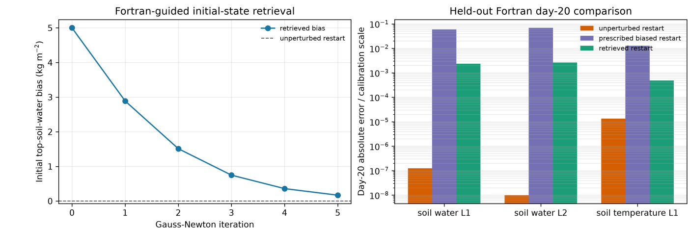
Figure B3. Fortran-guided initial-state retrieval using an autonomous offline SURF trajectory. Left: reverse-mode, damped Gauss–Newton recovery of the prescribed top-layer soil-water bias from the day-10 Fortran target. Right: normalized absolute errors against the held-out day-20 Fortran state. The unperturbed restart is shown only as a numerical-reference path and is not used to construct the retrieval target.
