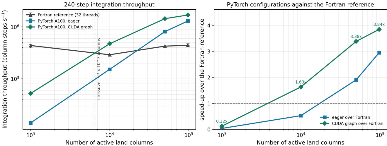
Figure 18. Integration throughput and accelerator speed-up for the autonomous offline SURF implementation over 240 continuous steps, against the Fortran reference on the same columns. Left: throughput for the Fortran reference and the A100 eager and CUDA-graph configurations; points are repeat medians, error bars span the observed minimum–maximum integration times. Right: each accelerator configuration’s speed-up over the Fortran reference.
