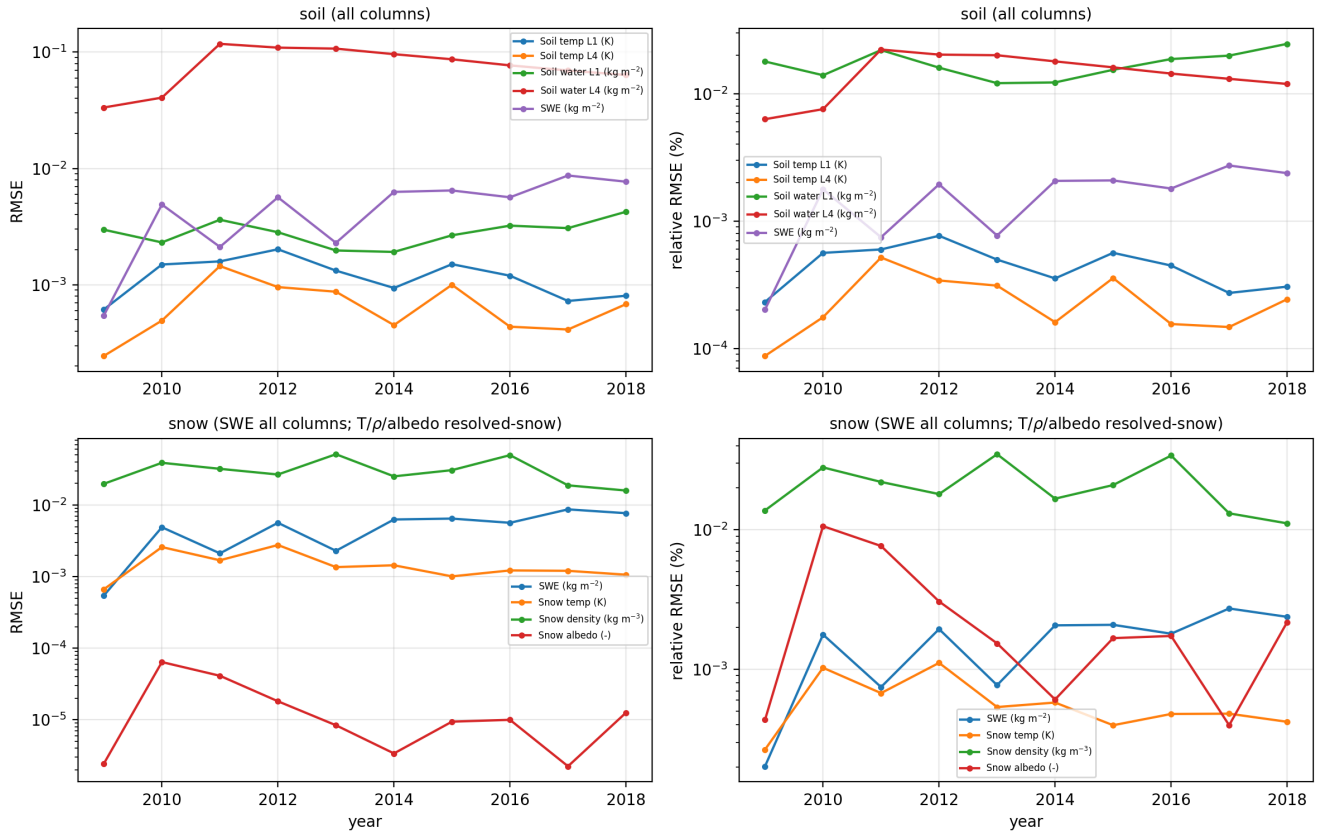
Decadal Fortran-PyTorch terminal errors, 2009–2018
