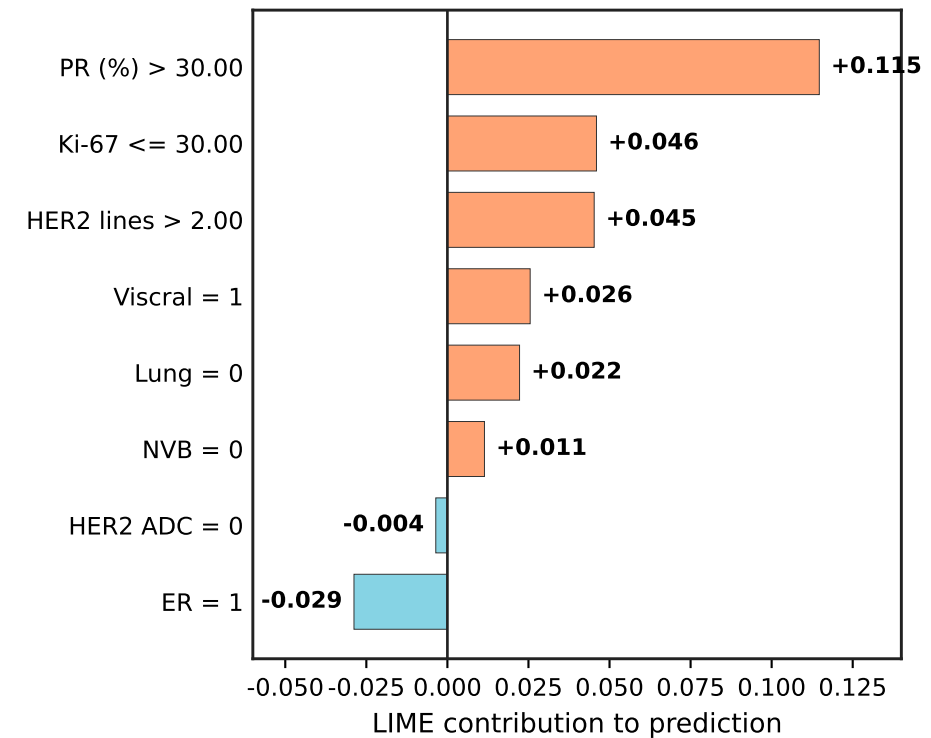
highest prediction | idx=3 \hat{y}=0.472
