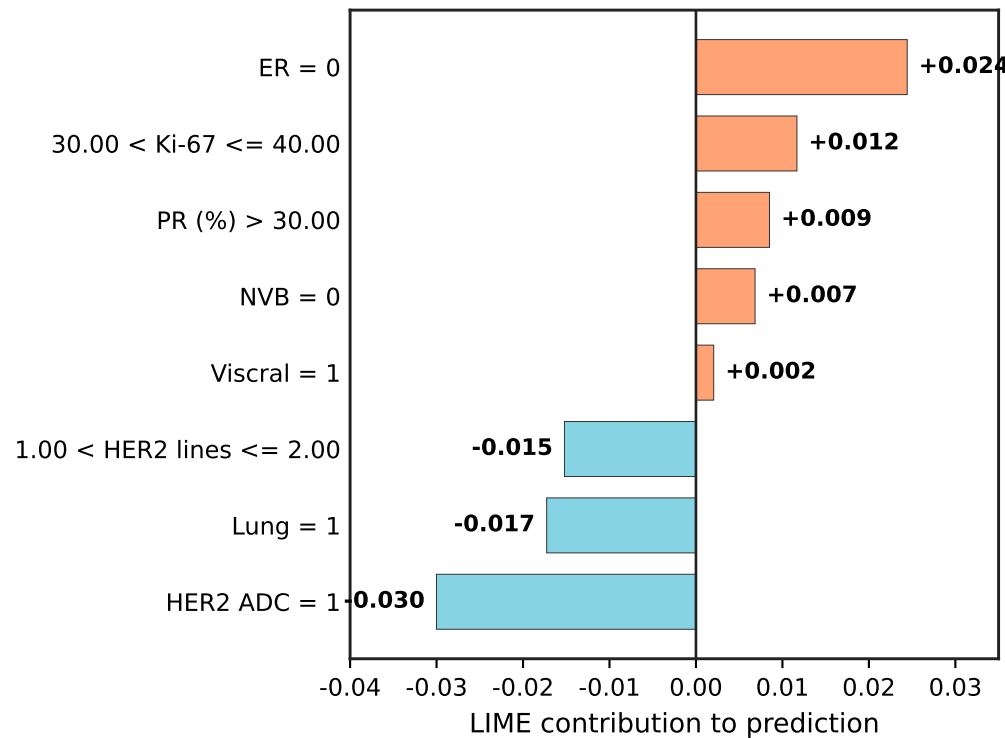
median prediction | idx=77 \hat{y}=0.230
