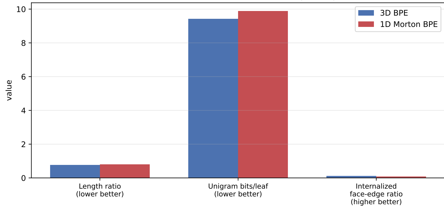
3D BPE vs 1D Morton BPE (same merge budget)
