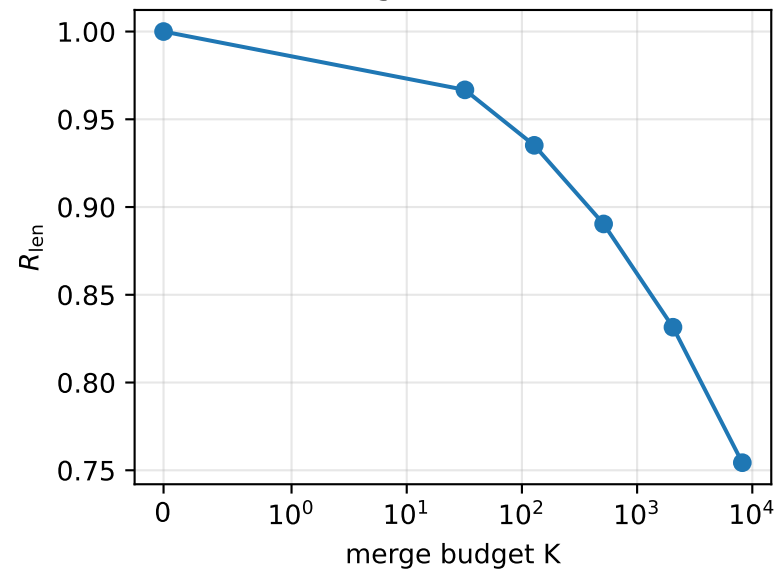
Length ratio vs K
