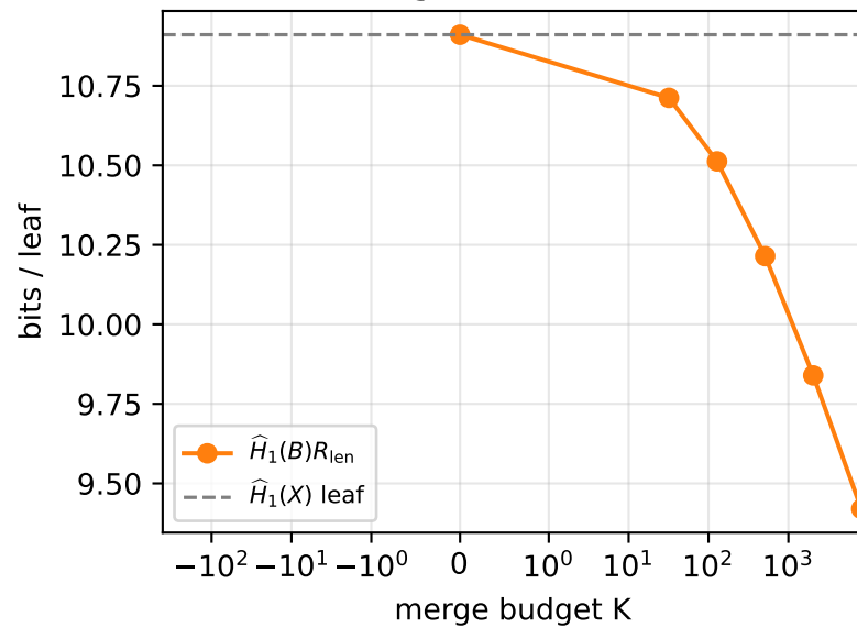
Unigram cost vs K
