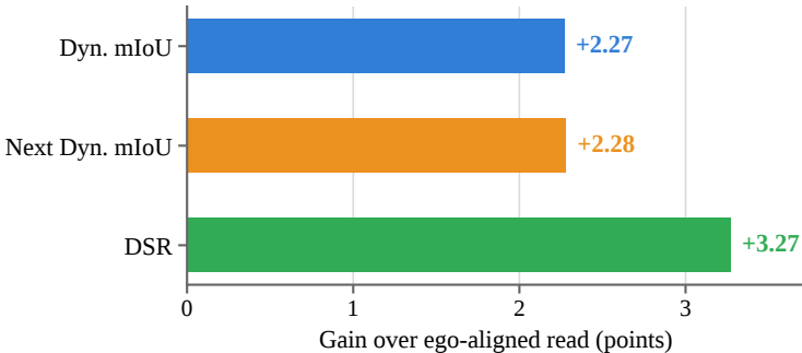
(a) Occupancy and coverage gains
