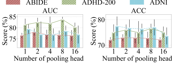
Figure 5. Impact of the number of pooling heads.
