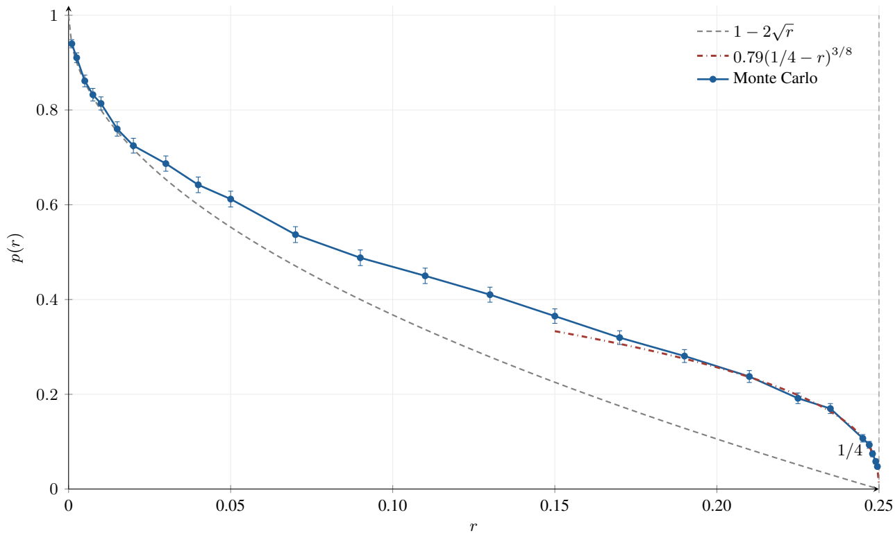
Limiting one-atomic probability
