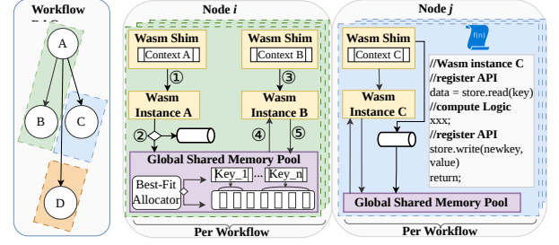
Figure 4: Intra-node execution architecture. Circled numbers trace the data path for co-located functions A and B; cross-node edges are forwarded to TCP push (§3.3).
