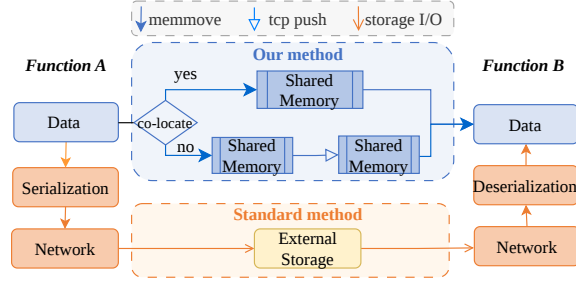
Figure 3: Data transfer path comparison. Standard method : 5 intermediaries, 2× serialization. Our method : local edges use SHM (2× memmove, 0× serialization); remote edges use TCP push (3× memmove, 0× serialization).
