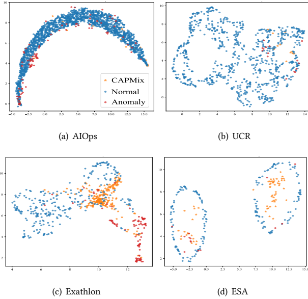
Figure 4: UMAP visualization of samples generated by CAP-Mix (orange), along with normal (blue) and real anomalous (red) test samples. CAPMix aligns better with real anomalies while largely avoiding overlap with normal regions.
