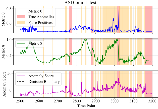
Figure 1: False alarms of a normality-assumption detector OC-SVM on a representative KPI stream. The top panels show raw KPI sequences, and the bottom panel shows the OC-SVM anomaly score. Benign system fluctuations are repeatedly flagged as anomalies (orange), obscuring true anomalies (red) and causing an excessive false-positive rate.
