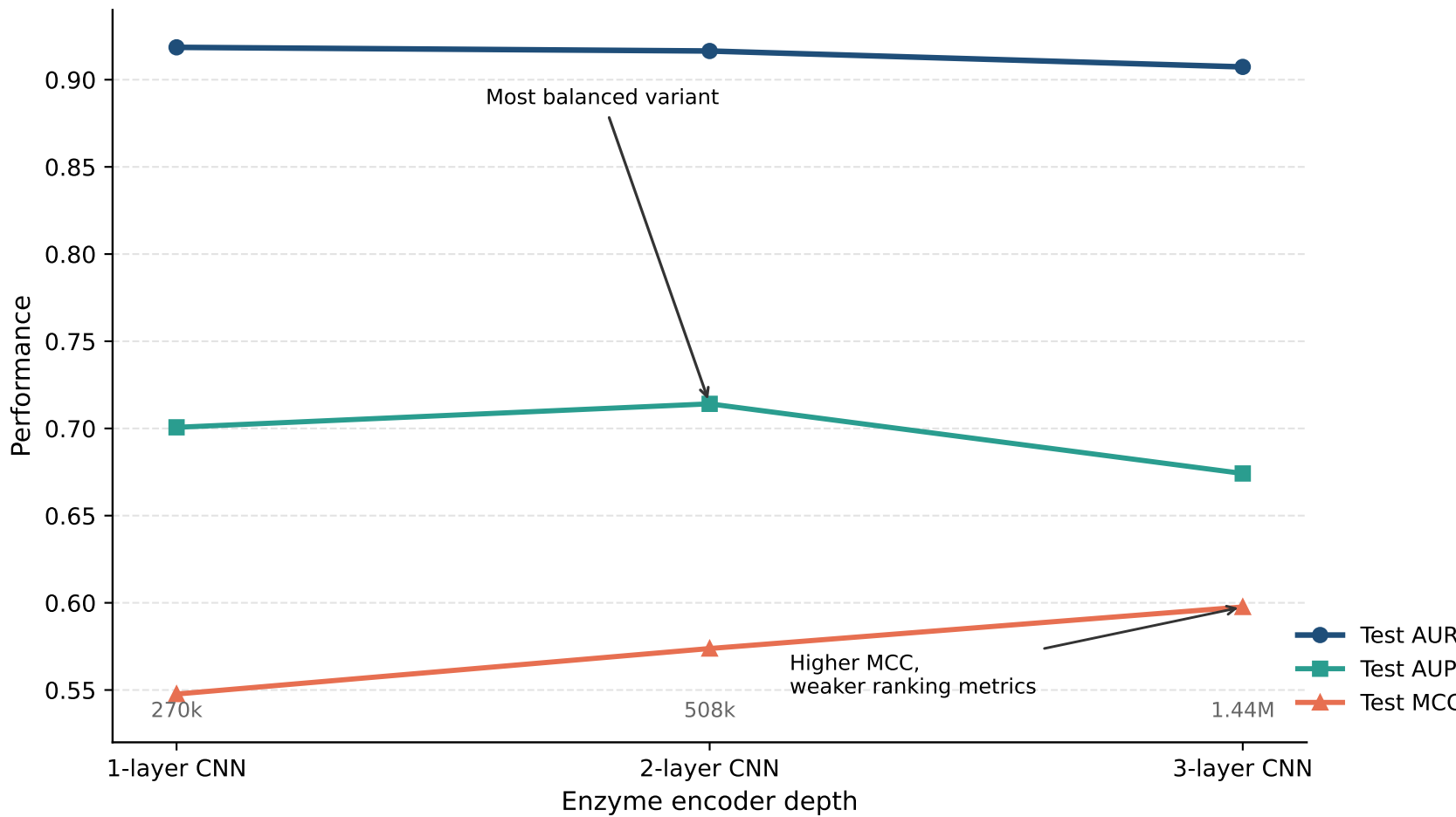
Figure 2. Enzyme-side CNN Depth Ablation Under Controlled Evaluation (Exp13)
