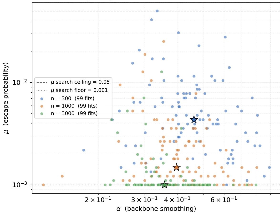
Fitted KRegCCD parameters — Yule50 (99 reps \times 3 sizes)
