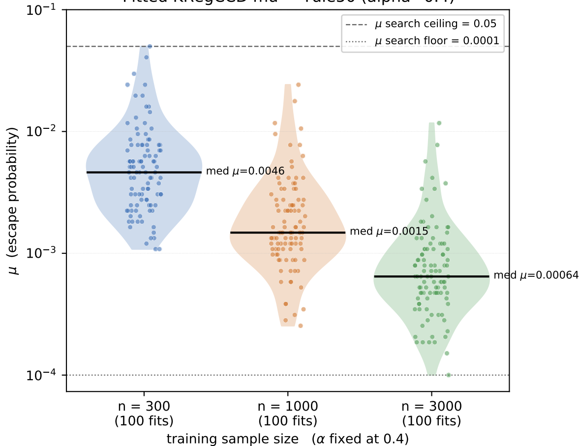
Fitted KRegCCD \mu — Yule50 ( \alpha=0.4 )
