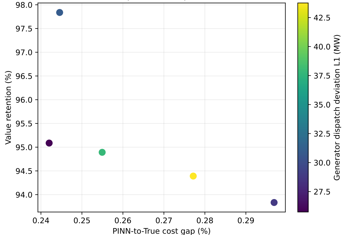
Economic impact and dispatch deviation
