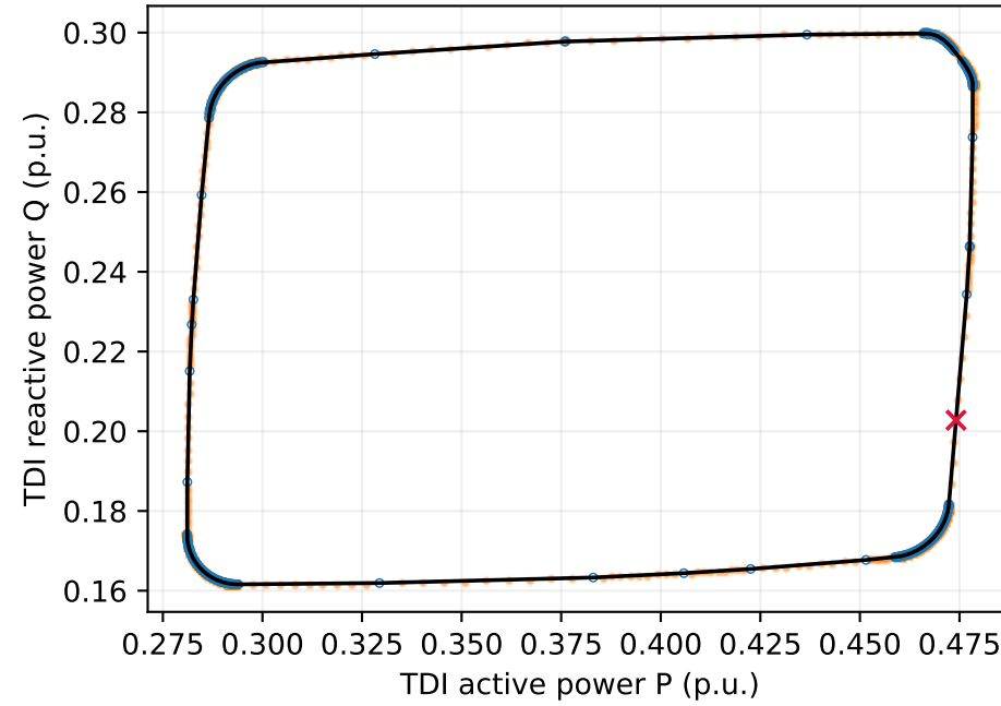
33-bus system (condition 10) max normalized distance = 0.0687%
