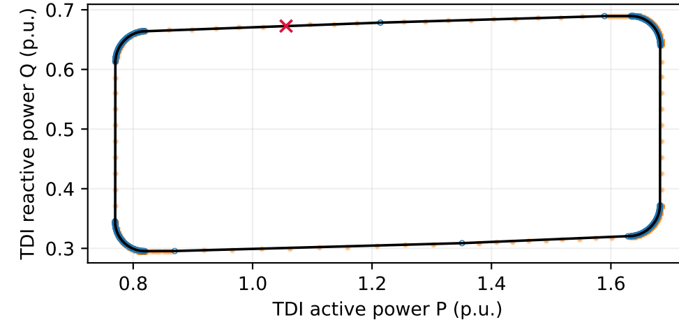
36-bus three-phase system (condition 7) max normalized distance = 0.0741%
