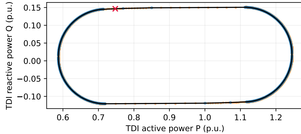
533-bus system (condition 8) max normalized distance = 0.0271%
