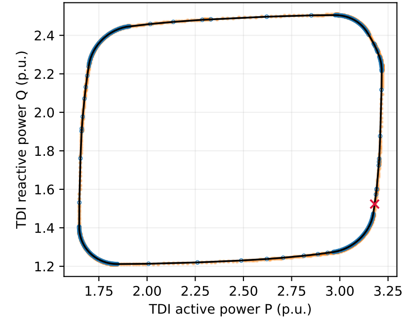
118-bus system (condition 2) max normalized distance = 0.0297%
