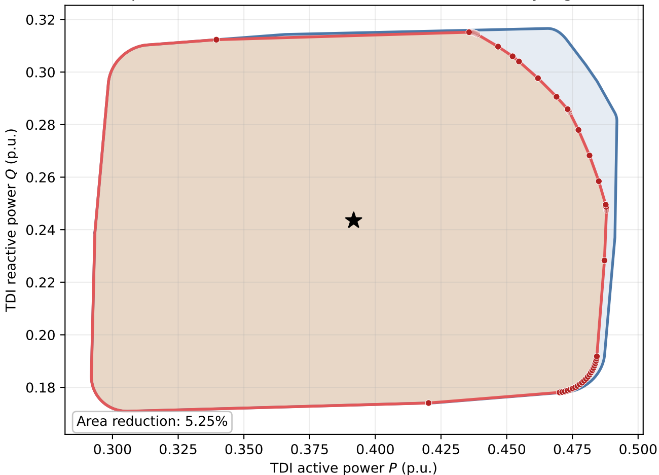
Impact of branch thermal limits on the true flexibility region
