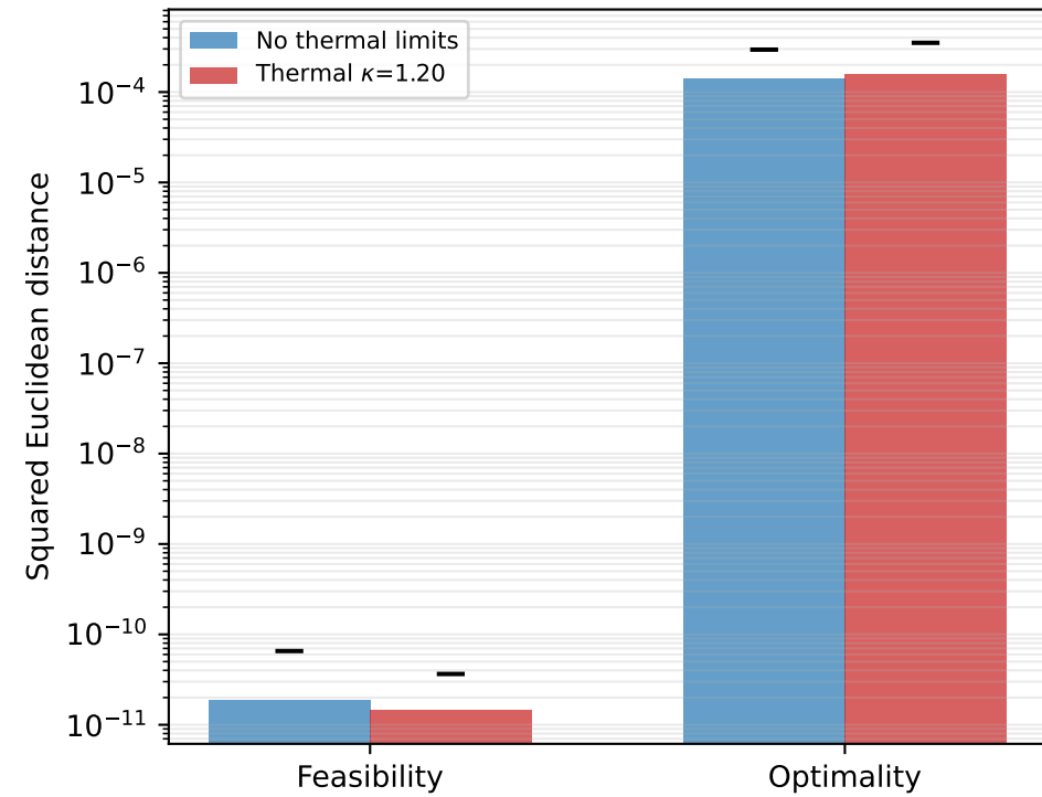
(c) Approximation errors (bar: mean; mark: P95)
