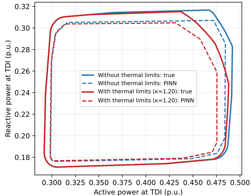
(a) Nominal flexibility regions
