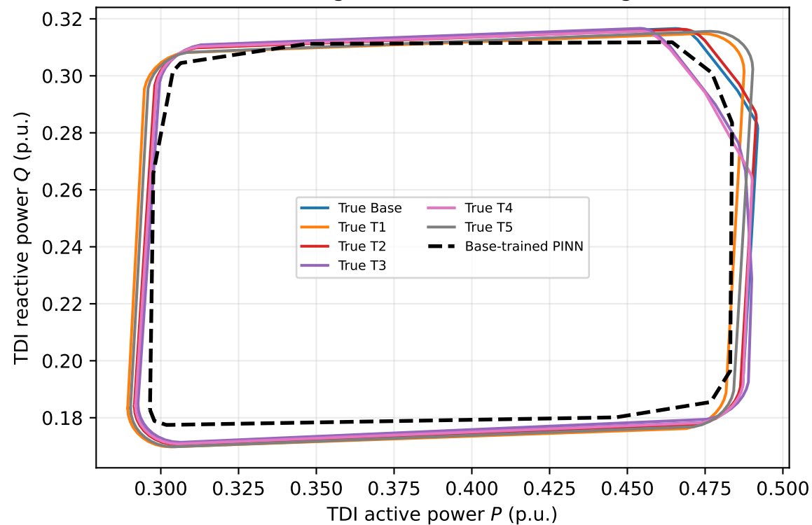
(a) Nominal regions under radial reconfiguration
