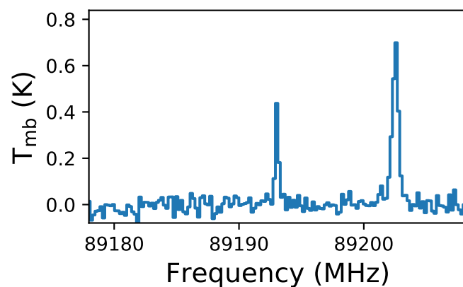
HCO+
