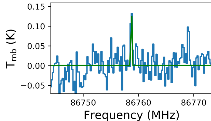
HCO+
