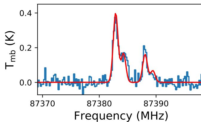
HCO +
