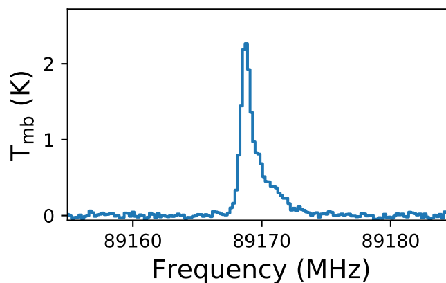
HCO +
