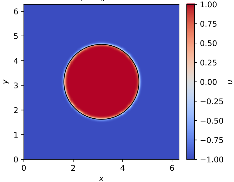
t = 50, \quad R_h = 1.5187
