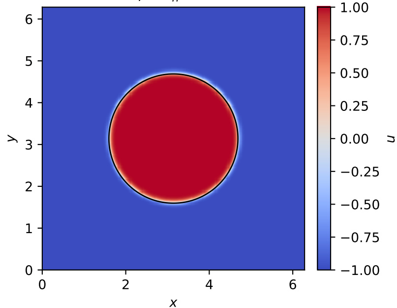
t = 100, \quad R_h = 1.4655
