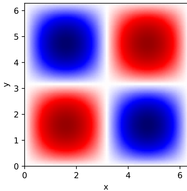
Exact \omega(T)
