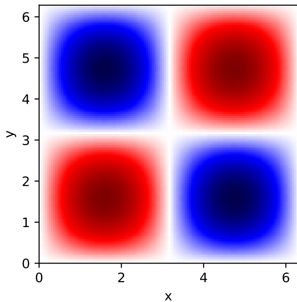
Exact \omega(T)
