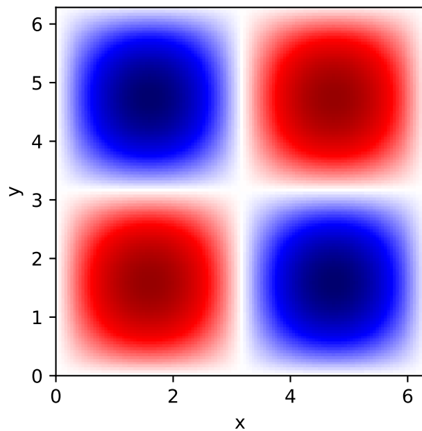
Pointwise error |\omega - \omega_{\text{ex}}|
