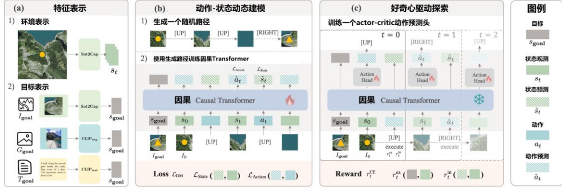
图 3. GeoExplorer 学习流程。学习过程可以依次分为三个阶段：特征表示、动作-状态动态建模 (DM) 和好奇心驱动探索 (CE)。(a) 特征表示：环境 ( S_t ) 和目标 ( S_{goal} ) 根据其模态（例如，航拍图像 ( I_{goal} )、地面图像 ( G_{goal} ) 或文本 ( T_{goal} )）使用不同但对齐的编码器进行编码。(b) 动作-状态动态建模：训练一个因果 Transformer 来联合捕捉动作-状态动态，由生成的动作-状态轨迹对环境建模提供监督。(c) 好奇心驱动探索：基于 (b) 中的状态预测，将好奇心驱动的内生奖励 ( r_t^{CE} ) 与基于距离的外在奖励 ( r_t^{in} ) 相结合，通过测量预测与观察之间的差异来鼓励智能体探索环境。(Figure 3. GeoExplorer learning pipeline. The learning process can be divided into three stages sequentially: Feature Representation, Action-State Dynamics Modeling (DM), and Curiosity-Driven Exploration (CE). (a) Feature Representation . The environment ( s_t ) and goal ( s_{goal} ) are encoded with different but aligned encoders, according to their modalities (e.g., aerial images ( I_{goal} ), ground-level images ( G_{goal} ), or text ( T_{goal} )). (b) Action-State Dynamics Modeling . A causal Transformer is trained to jointly capture action-state dynamics, guided by supervision from generated action-state trajectories for environment modeling. (c) Curiosity-Driven Exploration . Based on state prediction from (b), a curiosity-driven intrinsic reward ( r_t^{in} ) is combined with the distance-based extrinsic reward ( r_t^{ex} ) to encourage the agent to explore the environment by measuring the differences between prediction and observations.)
