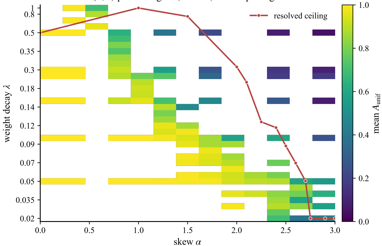
(\alpha, \lambda) phase diagram, n = 10 , 60k-step budget
