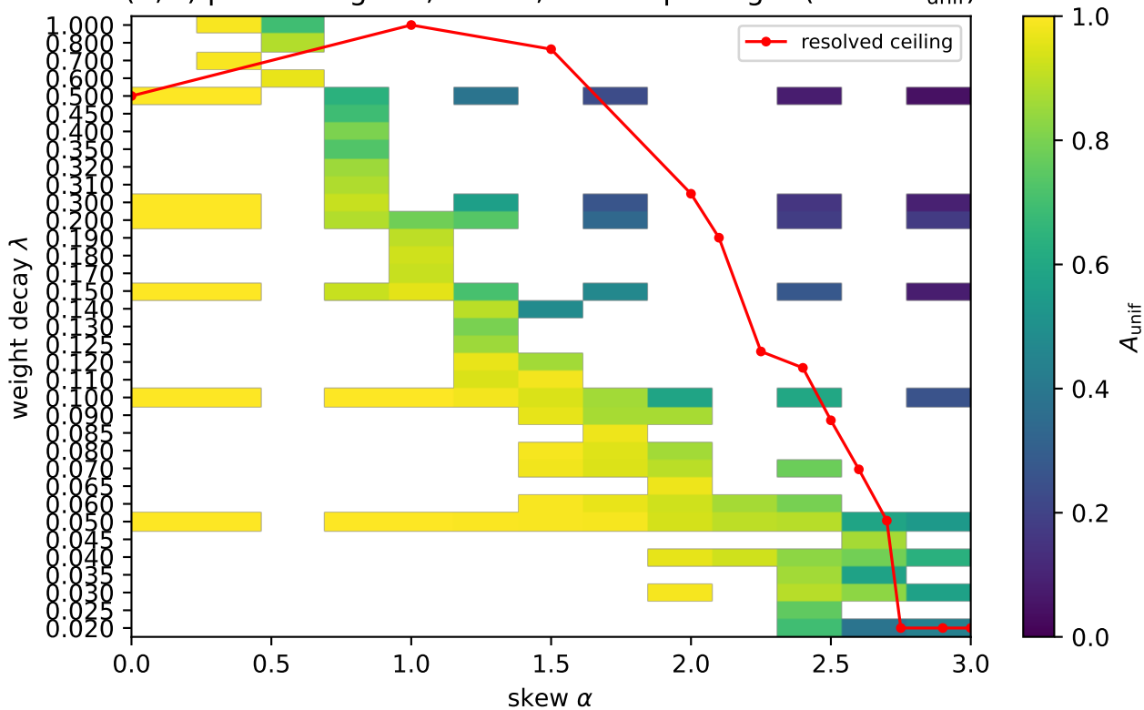
(\alpha, \lambda) phase diagram, n = 10 , 60k-step budget (mean A_{\text{unif}} )
