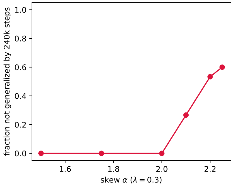
(a) censoring fraction
