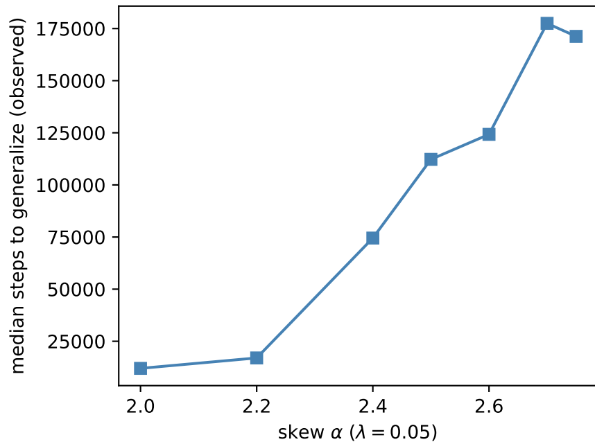
(b) median generalization time
