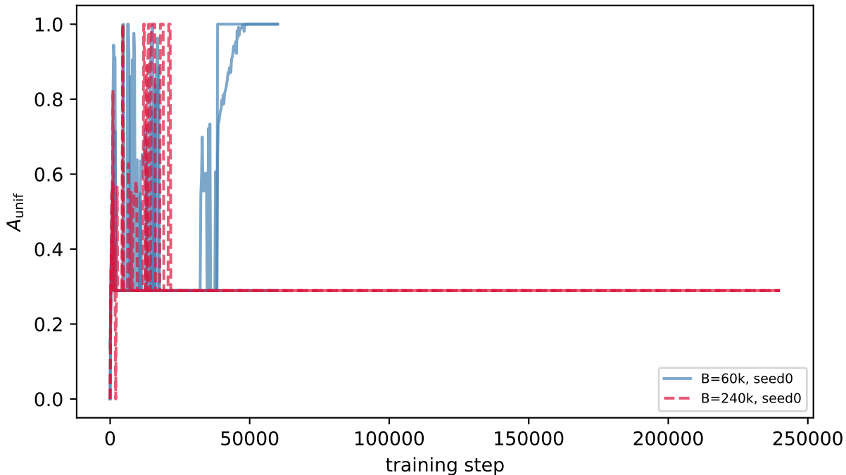
Dyck-1 shallow-grok metastability, \alpha = 6.0 , \lambda = 0.9
