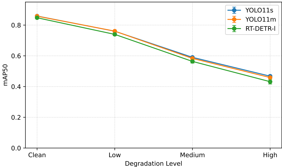
Robustness under Motion Blur
