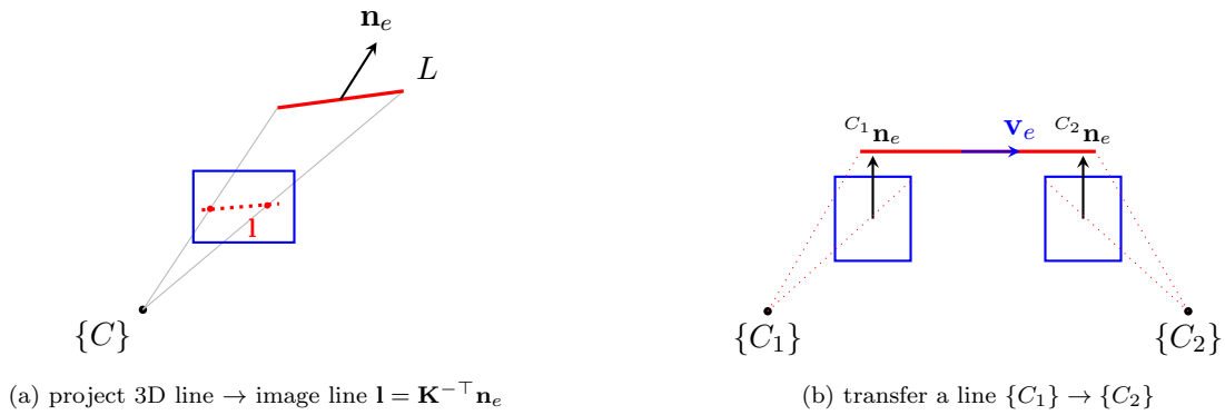
Figure 11: Lines with cameras: projecting a 3D line to a 2D image line (a) and transferring a line between two camera frames (b).
