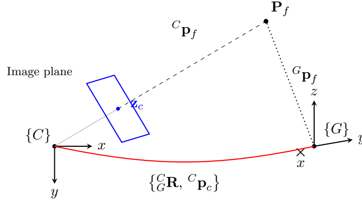
Figure 4: Camera measurement geometry: the feature \mathbf{P}_f projects through the image plane to the pixel \mathbf{z}_c in the camera frame \{C\} ; the global frame \{G\} and the extrinsic \{^C_G\mathbf{R}, ^C\mathbf{p}_c\} relate the two views of the same point ( ^C\mathbf{p}_f vs. ^G\mathbf{p}_f ).
