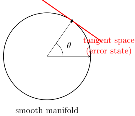
Figure 3: A smooth manifold (here a circle/sphere) avoids the wrap-around of a raw angle; the red tangent line is the local vector space used to model derivatives and error states for optimization.
