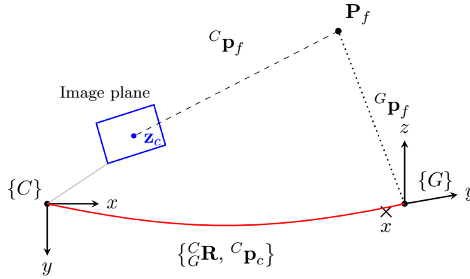
Figure 4: Camera measurement geometry: the feature \mathbf{P}_f projects through the image plane to the pixel \mathbf{z}_c in the camera frame \{C\} ; the global frame \{G\} and the extrinsic \{^C_G \mathbf{R}, ^C \mathbf{p}_c\} relate the two views of the same point ( ^C \mathbf{p}_f vs. ^G \mathbf{p}_f ).
