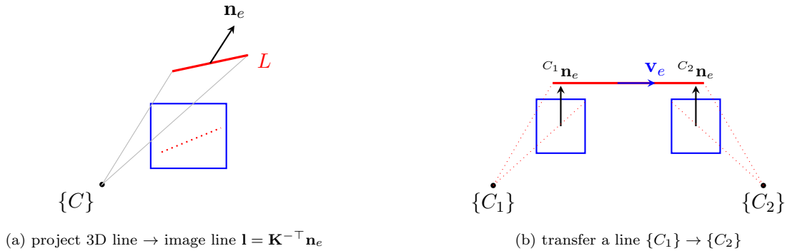
Figure 11: Lines with cameras: projecting a 3D line to a 2D image line (a) and transferring a line between two camera frames (b).
