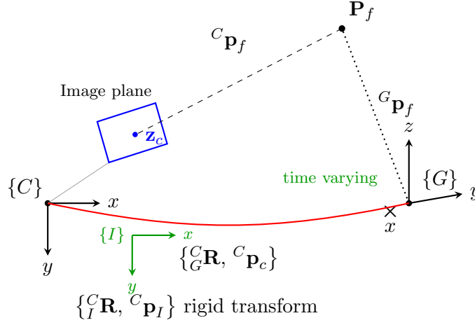
Figure 8: Extrinsic calibration: the IMU frame \{I\} is rigidly fixed to the camera \{C\} via \{^C_I \mathbf{R}, ^C_I \mathbf{p}_I\} , while the camera-to-global transform is time varying.
