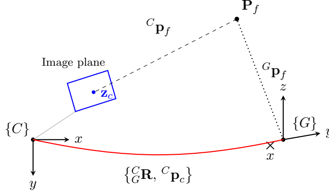
Figure 7: The intrinsic calibration sits inside the same projection geometry: the 3D feature is transformed into \{C\} , projected, distorted, and mapped to pixels.
