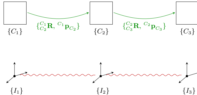
Figure 17: Visual-inertial initialization: the relative camera poses from the visual SLAM pipeline (top, green) are aligned with the IMU integration over the same intervals (bottom, red wavy links) through the camera–IMU extrinsics.
