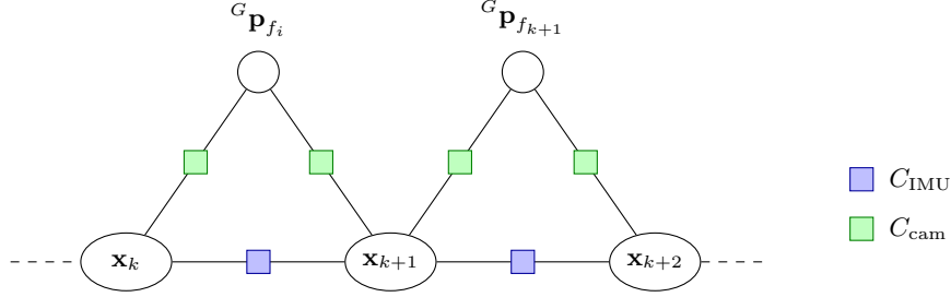
Figure 19: Factor graph of an optimization-based VINS: pose/navigation states \mathbf{x}_k are linked by IMU (preintegration) factors, and to the features {}^G\mathbf{p}_f by camera factors.
