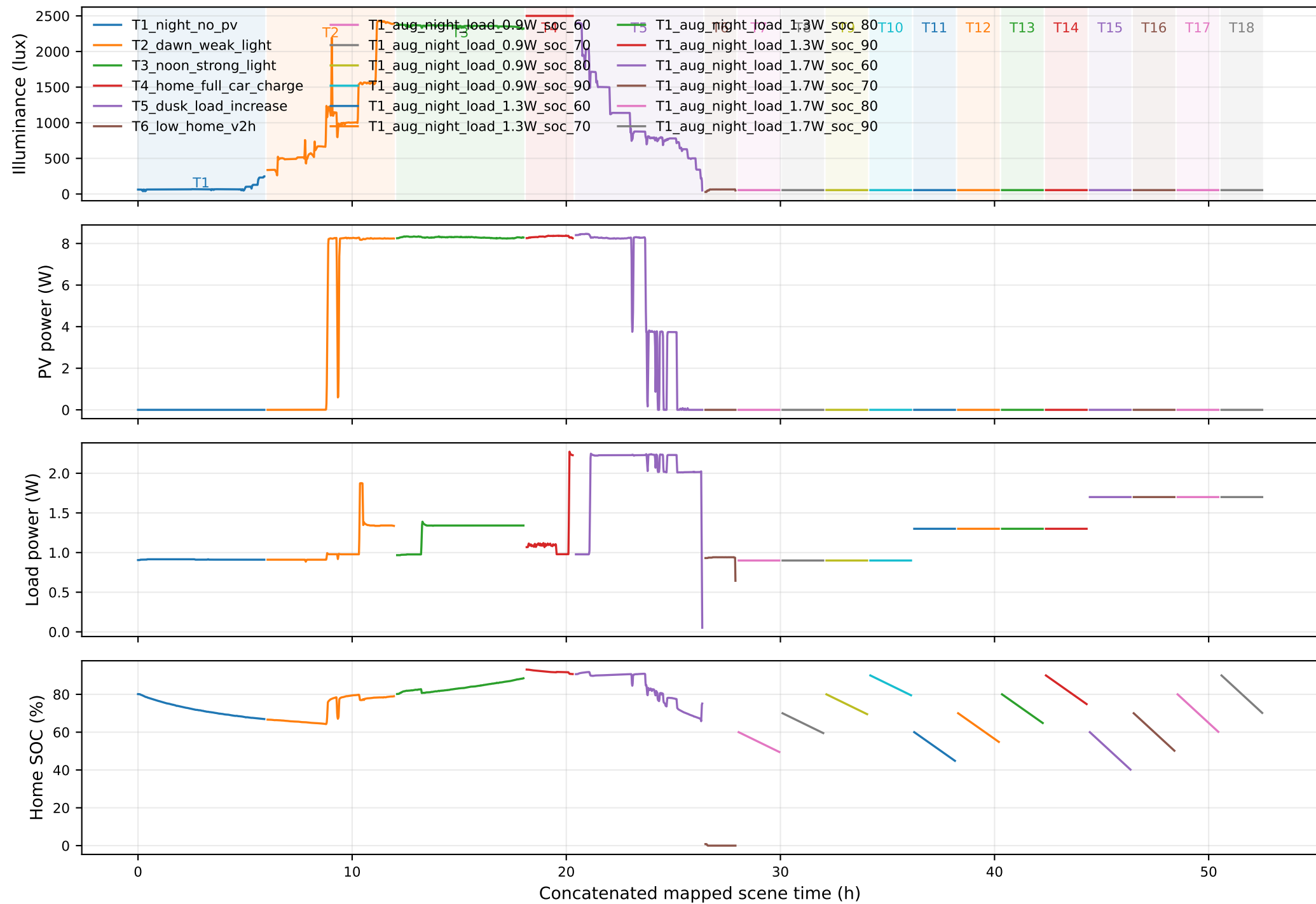
Energy-dispatch dataset under six representative scenarios
