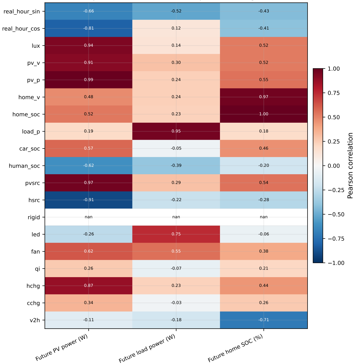
Input-feature correlation with prediction targets
