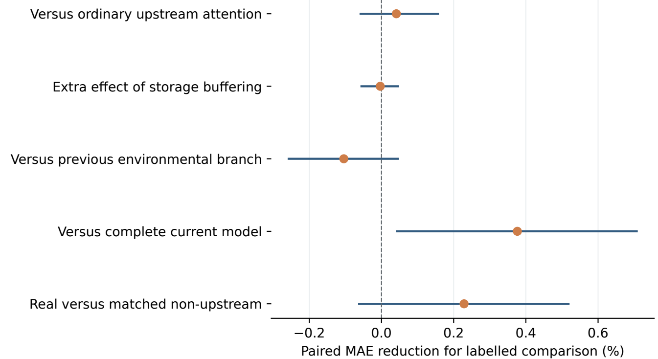
b Overall DOC reconstruction
