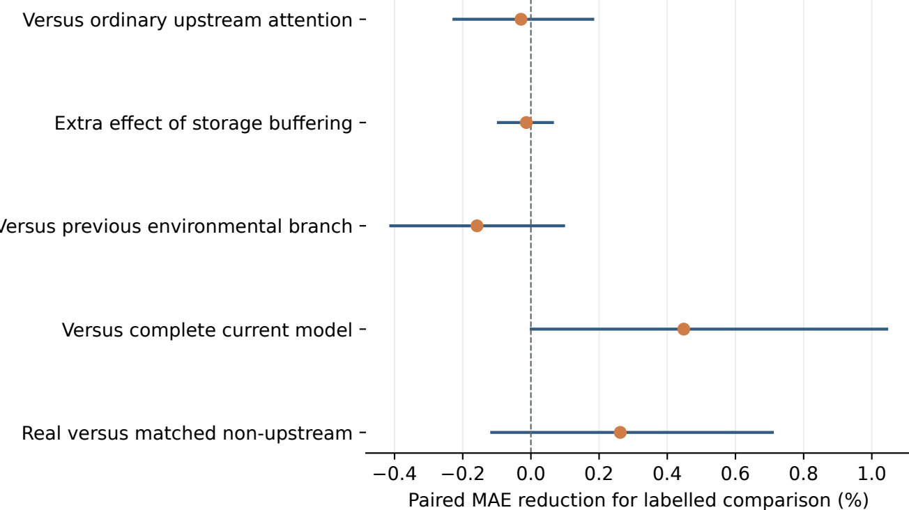
c Source-Q90 high-DOC reconstruction
