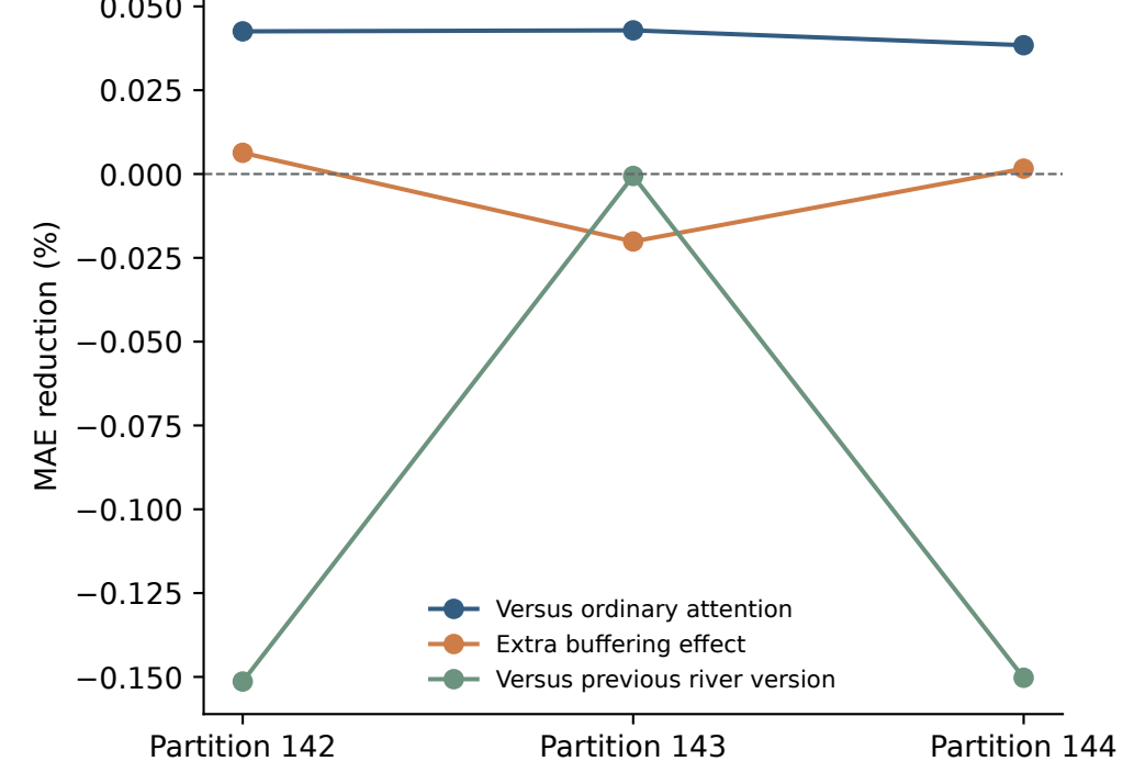
d Three-partition stability
