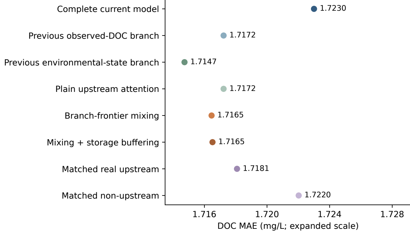
a Same receiving cells and frozen local model
