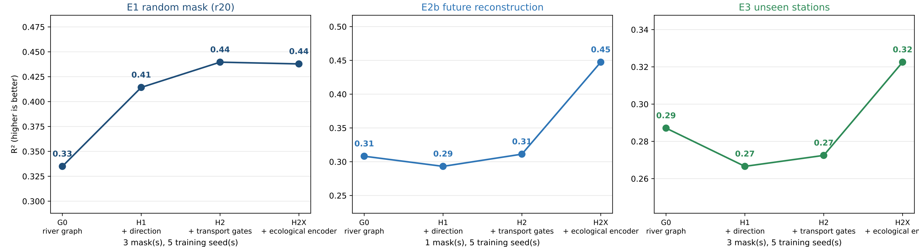
Figure 1 | Stored model performance across scenarios ( R^2 , equal-weight mean over each scenario's masks)
