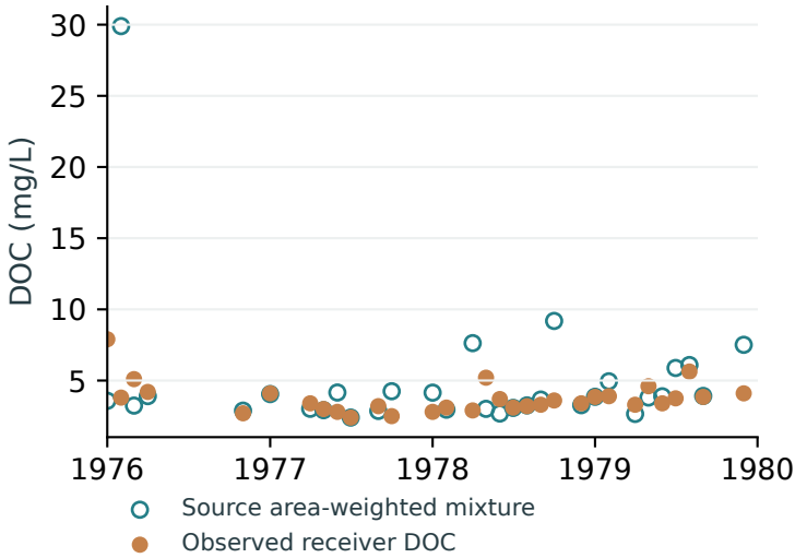
f Actual common sampling months 2 inputs; 31 months; median sample span 8 days
