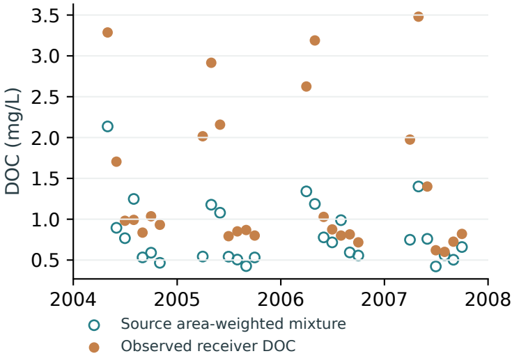
e Actual common sampling months 2 inputs; 28 months; median sample span 0 days
