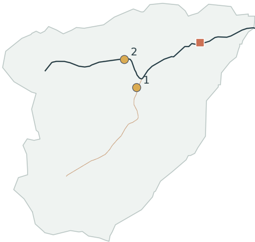
b Mainstem dominated 401733105392404 · area coverage 75%
