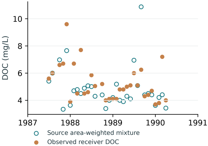
d Actual common sampling months 2 inputs; 32 months; median sample span 2 days
