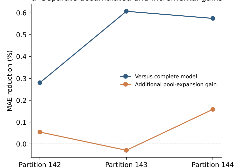
d Separate accumulated and incremental gains
