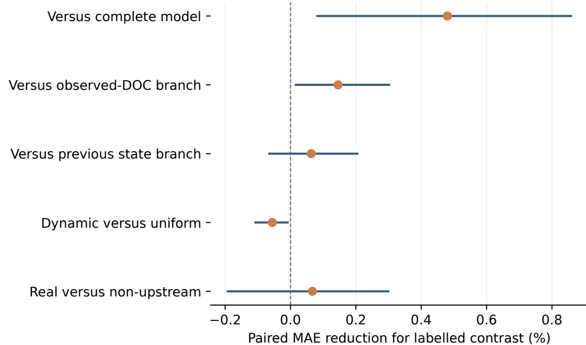
b Paired station intervals (5,000 draws)
