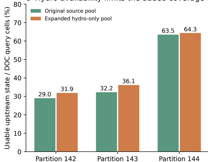
c Hydro availability limits the added coverage
