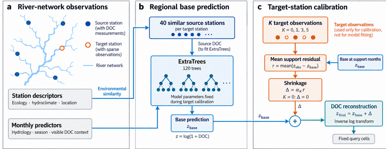
Figure 1: Regional prediction with sparse station residual calibration. a , Station descriptors select environmentally similar sources; monthly predictors include visible DOC context from the river network. b , A target-specific ExtraTrees model is fitted on 40 source stations and then held fixed. c , Target observations estimate a shrunk mean residual in \log(1 + \text{DOC}) space. This correction is added to the base prediction before inverse transformation and nonnegative clipping. At K = 0 the correction is zero. Support labels enter only calibration; query labels enter only evaluation. River branches and tree icons are schematic.
