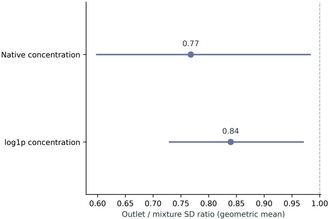
a Outlet variability depends on scale
