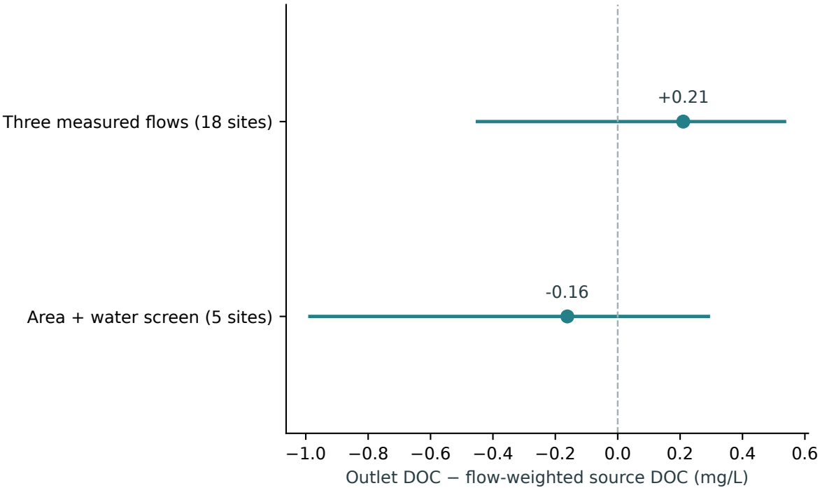
b Apparent departure does not establish channel loss
