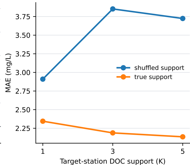
C Support-label diagnostic
