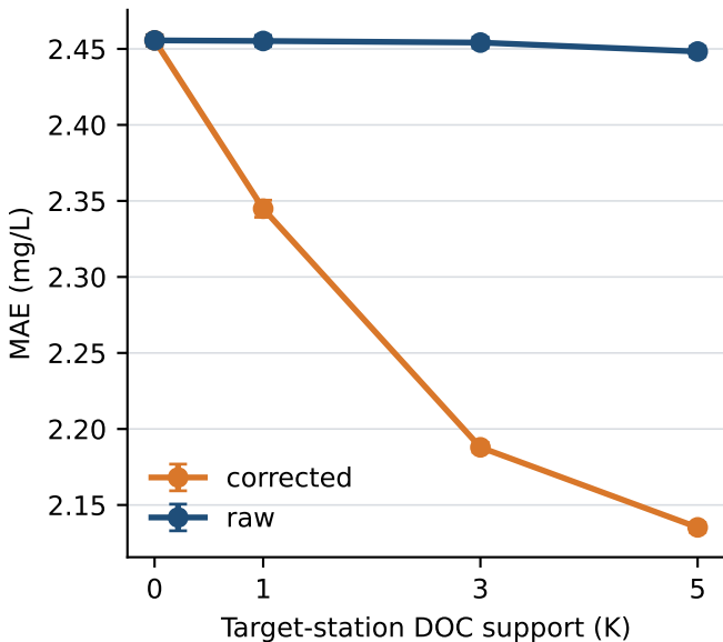
A Fixed-query reconstruction curve
