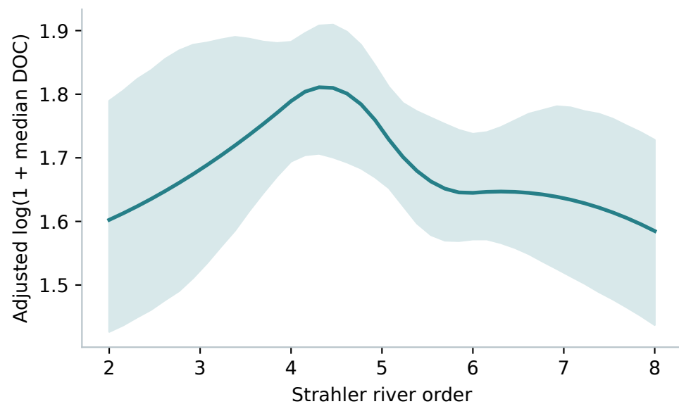
River order
