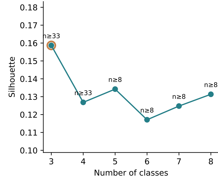
b Data-derived class count
