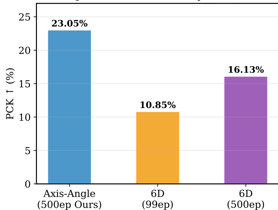
Joint Position Accuracy (PCK)
